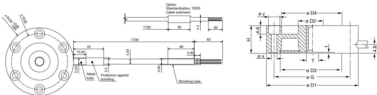
Dimensional drawing 2 – Measuring ranges from 0 ... \pm 5 kN up to 0 ... \pm 10 kN | from 0 ... \pm 1.1 klbs up to 0 ... \pm 2.2 klbs
